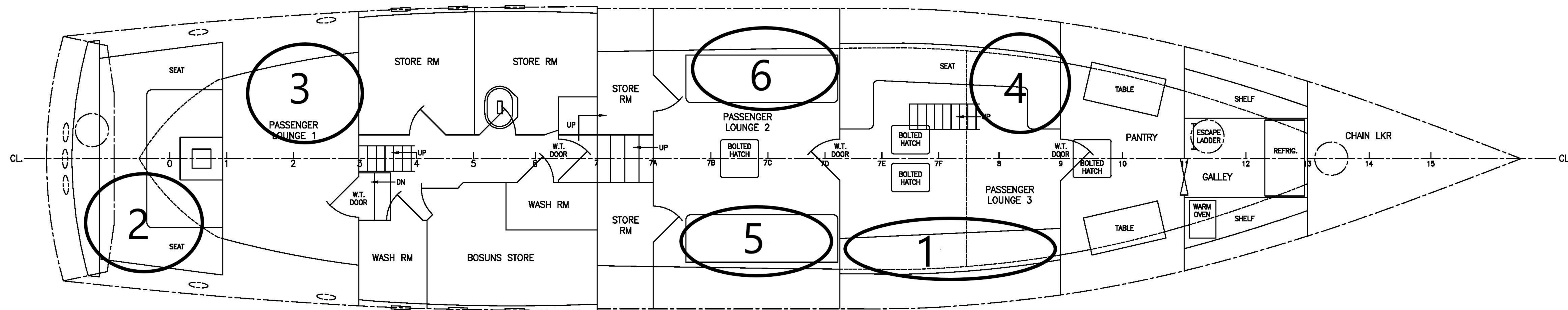
PLAN AT LOWER DECKS
